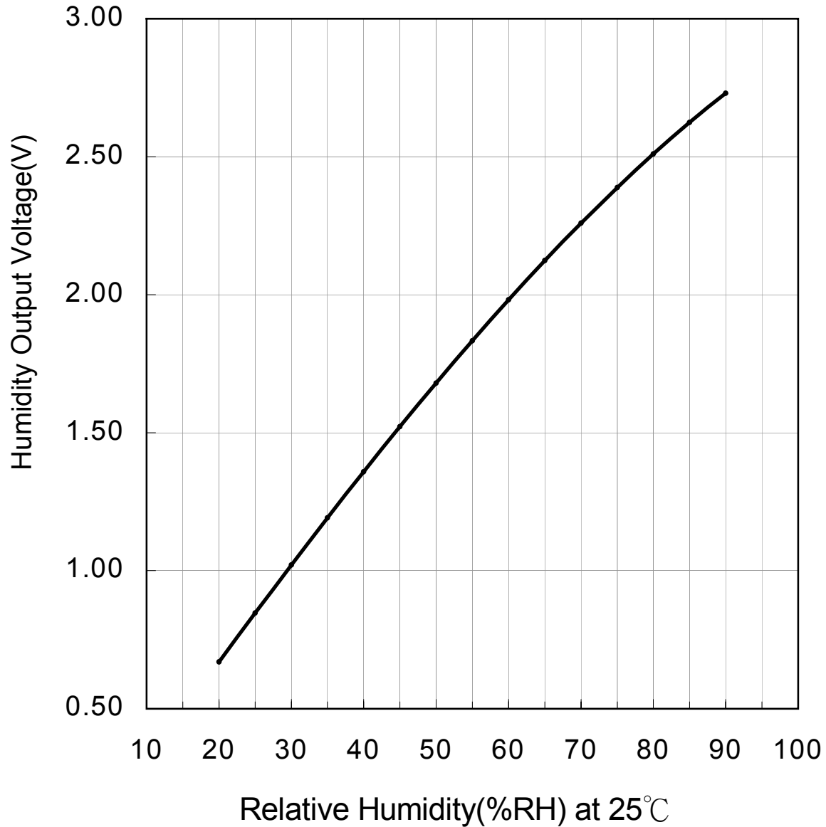
HMZ-333A1 Humidity Output 0~3.3V characteristics
